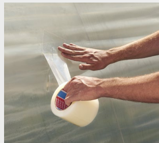
Step 2: Apply tesa® 4646 on a dry and clean surface
